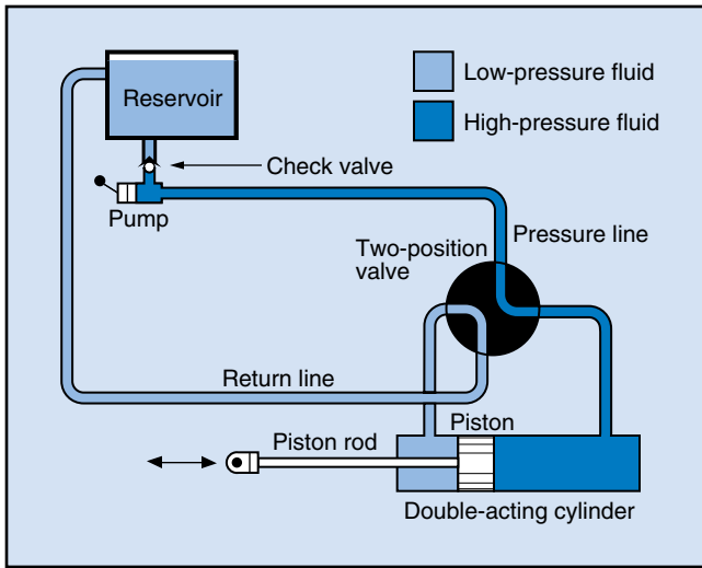
Fig. 1-12. A basic hydraulic system
