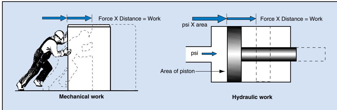
Fig. 1-3. Comparison between hydraulic and mechanical work
