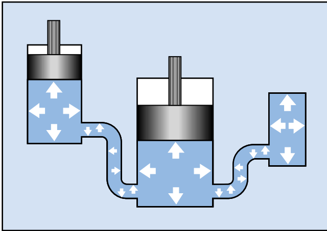
Fig. 1-6. Transmission of fluid pressure
