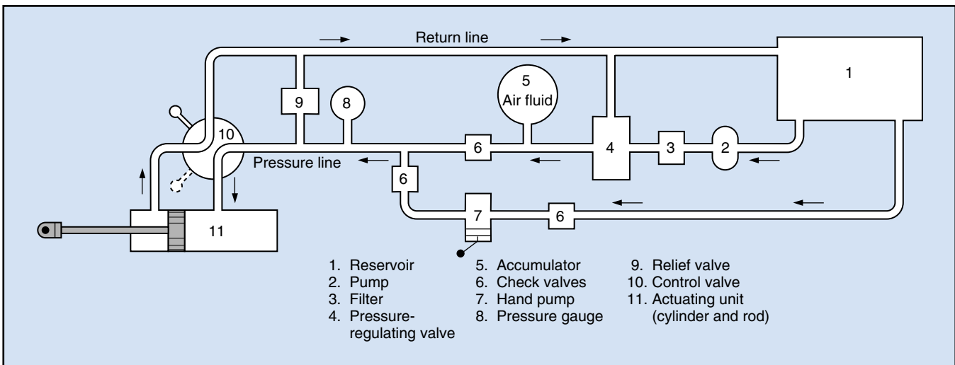
Fig. 1-13. A basic hydraulic system with accessories
