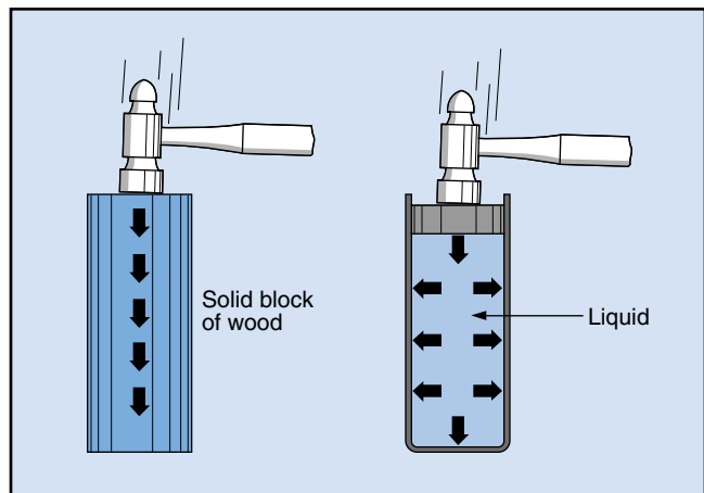
Fig. 1-5. Pascal's Law
