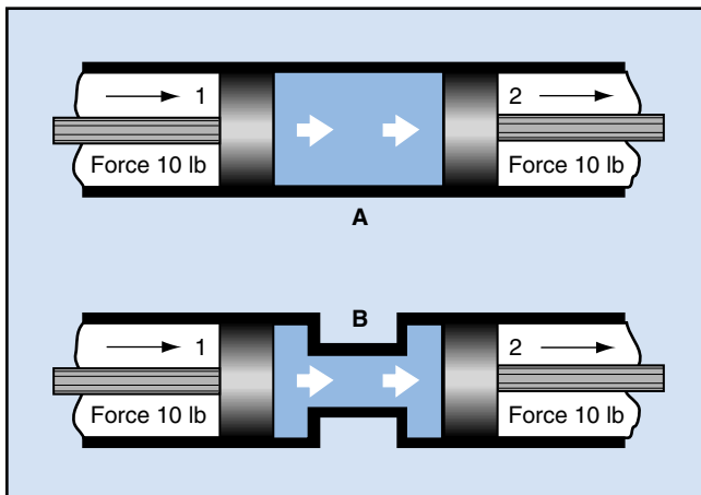
Fig. 1-7. Transmission of force
