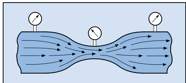
Fig. 1-11. A gradual piping constriction
